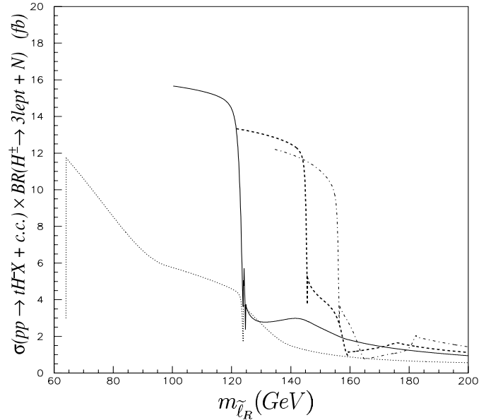
Fig. 5. \sigma(pp \rightarrow tH^-X + \text{c.c.}) \times \text{BR}(H^\pm \rightarrow 3\ell N) (in fb), where \ell = e^\pm or \mu^\pm and N represents invisible final state particles, versus m_{\tilde{\ell}_R} , the soft slepton mass input for the first two generations (soft stau mass inputs are pushed up by an additional 100 GeV, A_\tau = 0 ). The set (M_2, \mu) is fixed at (210 GeV, +135 GeV) for Parameter Set A (solid curve), at (280 GeV, +150 GeV) for Parameter Set B (thick dashed curve) and at (300 GeV, -150 GeV) for Parameter Set C (dot-dashed curve). The dotted curve replaces m_{\tilde{\ell}_L} = m_{\tilde{\ell}_R} in Parameter Set A with m_{\tilde{\ell}_L} = m_{\tilde{\ell}_R} + 100 GeV. The curves are terminated at the left where they would be LEP2 excluded, including the additional condition that m_{\tilde{\nu}} > m_{\tilde{\chi}_1^0} ; \ell s from tau decays are included
