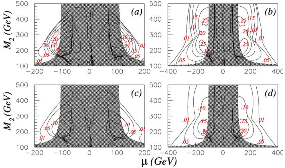
Fig. 2a–d. \text{BR}(H^\pm \rightarrow 3\ell N) , where \ell = e^\pm or \mu^\pm and N represents invisible final state particles, with (m_A, \tan\beta) = (a) (300 GeV, 10), (b) (500 GeV, 10), (c) (300 GeV, 20), (d) (500 GeV, 20). Slepton mass inputs are optimised as in the upper plots of Fig. 1. The shaded areas are excluded by LEP; m_t = 175 GeV, m_b = 4.25 GeV
