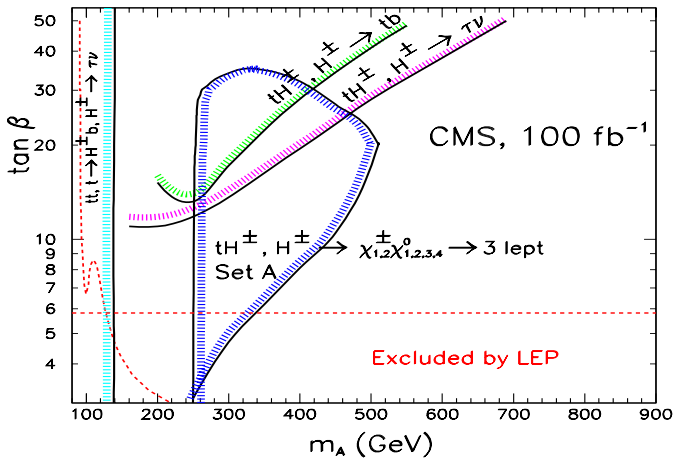
Fig. 9. 5\sigma discovery contours in the \tan\beta versus m_A plane for all charged Higgs channels, both SM and MSSM, assuming MSSM inputs as in Parameter Set A and 100\text{ fb}^{-1} of integrated luminosity. The area below the red dotted line at the left is excluded by LEP2 Higgsstrahlung (i.e., e^+e^- \rightarrow hZ and e^+e^- \rightarrow hA ) limits and the region below the horizontal red dotted line is excluded by the LEP2 chargino mass bound
